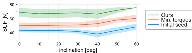
Fig. 4: Mean and standard deviation of the SUF at the end-effector for varying inclinations on the “ramp” scenario.
