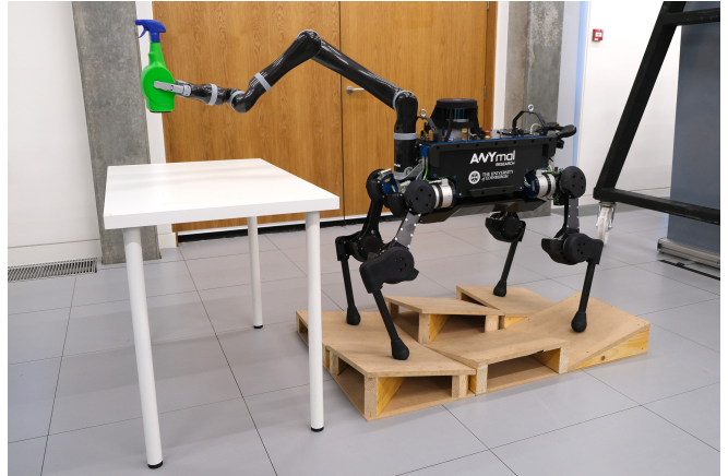
Fig. 1: A legged loco-manipulation system: ANYmal [2] is a fully torque-controlled quadruped robot. We equipped it with a Kinova Jaco [3] robot arm. An accompanying video is available at https://youtu.be/vDesP7IpThw .
